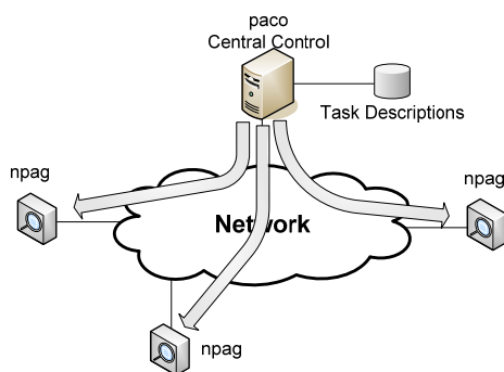
Figure 2. Architecture of paco
