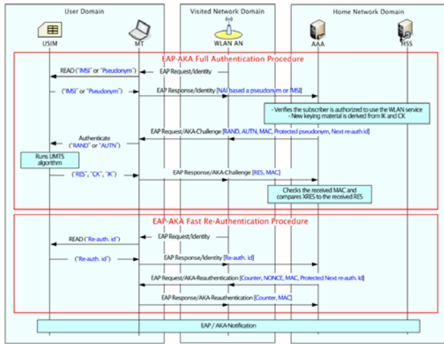
Fig. 3. EAP-AKA authentication Procedure
