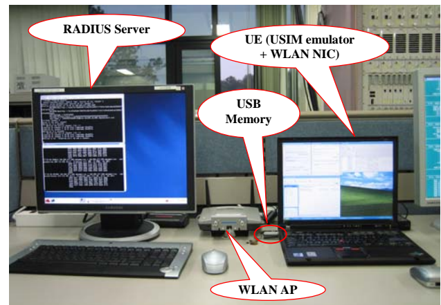
Fig. 6. Configuration of authentication test-bed
