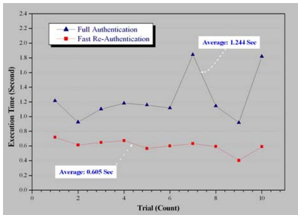
Fig. 9. Average authentication processing time
