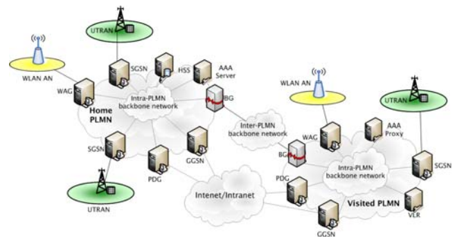
Fig. 1. UMTS-WLAN Overlay Network Model
