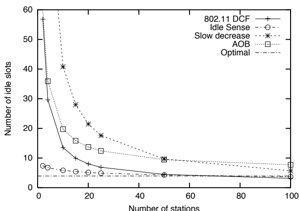
Fig. 5. Average number of consecutive idle slots between two transmission attempts, BER = 10^{-4}
