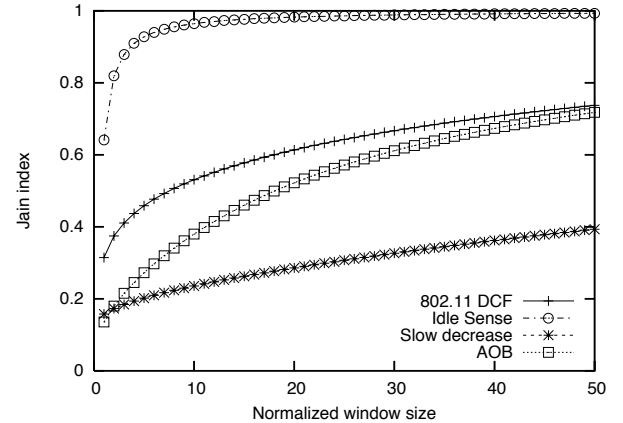
Fig. 3. Fairness comparison for 25 competing stations, BER = 10^{-5}
