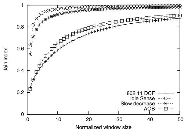
Fig. 6. Fairness comparison for 25 competing stations, BER = 10^{-4}
