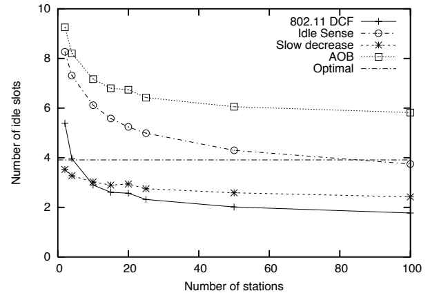
Fig. 2. Average number of consecutive idle slots between two transmission attempts, BER = 10^{-5}
