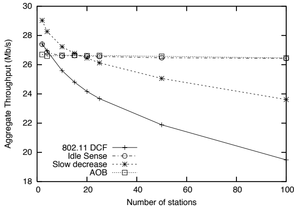
Fig. 1. Aggregate throughput vs. number of stations, BER = 10^{-5}
