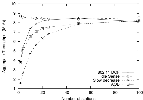
Fig. 4. Aggregate throughput vs. number of stations, BER = 10^{-4}
